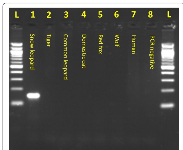
Figure 4 Snow leopard species identification PCR assay specificity. Snow leopard-specific PCR assay results showing amplification in only the snow leopard sample and complete lack of amplicons in other species assayed. The bottom two bands in the ladder are 100 bp and 200 bp, respectively.
